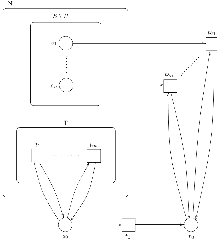
Figure 3.4: Construction of Theorem 3.2.25
