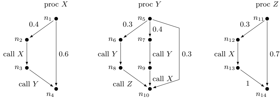
Fig. 2. Probabilistic flowgraphs
