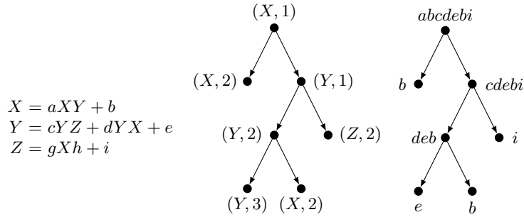
Fig. 3. A system of equations, a derivation tree, and its yield
