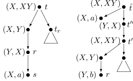
Figure 4: Transforming a derivation tree into a bamboo over a lossy semiring.
