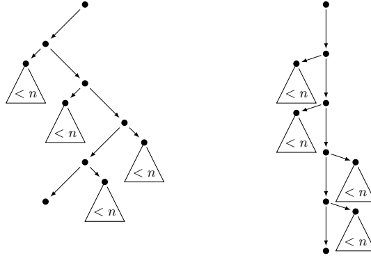
Figure 2: An example of the structure of a bamboo: it consists of a stem of unbounded length from which subtrees of height less than n sprout; on the right it is shown with its stem straightened.
