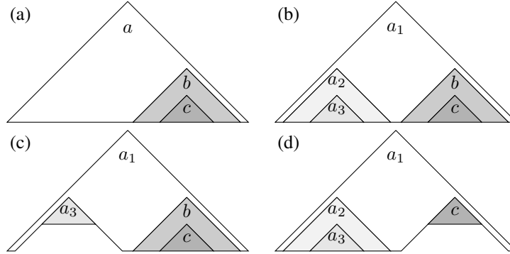
Figure 3: “Unpumping” trees to make them bamboos
