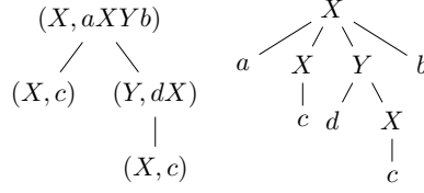
Figure 1: A derivation tree on the left, and its standard representation on the right
