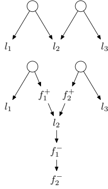
Figure 8: Transforming a 1-bounded STG into a 1-bounded free-choice STG
