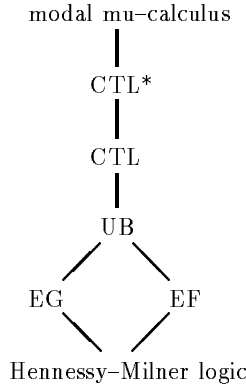
Fig. 2 Branching time logics
